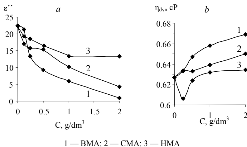
Figure 4. The concentration effect of amine-containing surfactants on the dipole-segmental coefficient (a) and the dynamic viscosity (b) of polyphenylsiloxane solutions ( C=0.5 \text{ g/dm}^3 ) at T=298 \text{ K}
